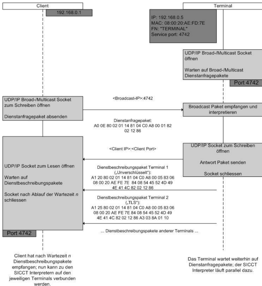
Abbildung 7 Service Discovery Broadcast
