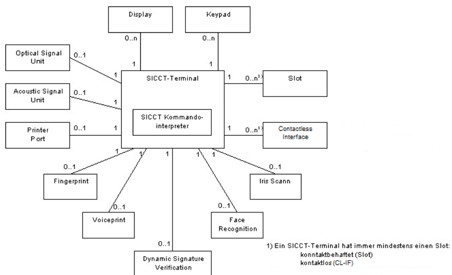
Abbildung 2: SICCT Functional Units
